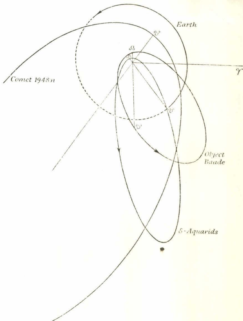
FIG. 135. The orbit of the \delta -Aquarid stream, computed from the radio-echo observations by Miss Almond. The orbits of comet 1948 n and of Baude's object 1566 Icarus are shown for comparison. Projection is on the plane of the ecliptic.
